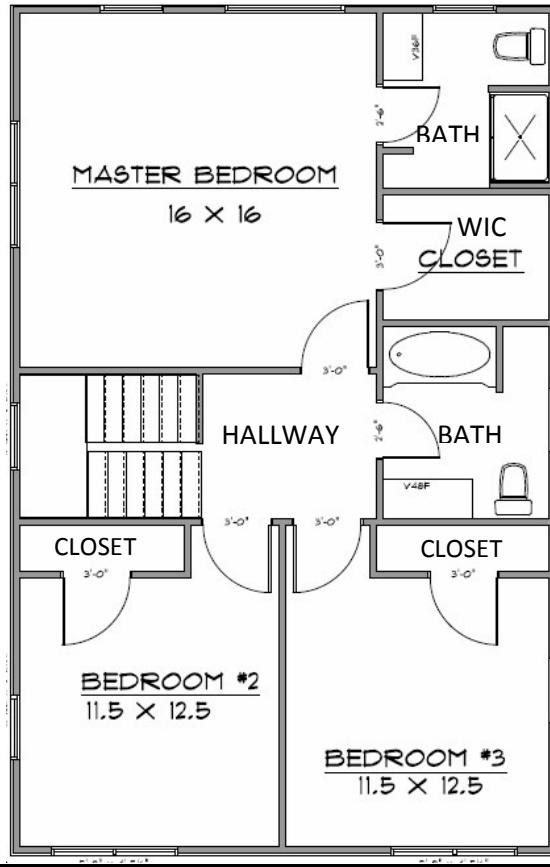
SECOND FLOOR FRONT OF HOUSE
